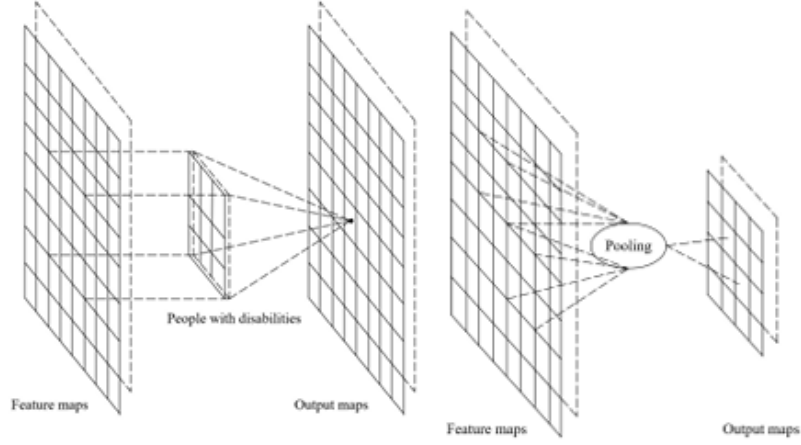
(a) CNN architecture
